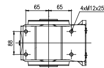
Shaft-mounted A
