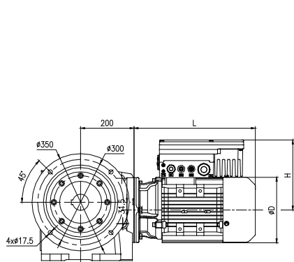
Flange-mounted F
