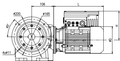
Flange-mounted F
